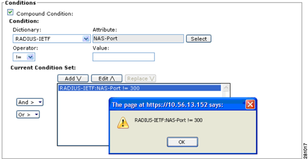
Figure 10-2 Compound Expression - Atomic Condition
